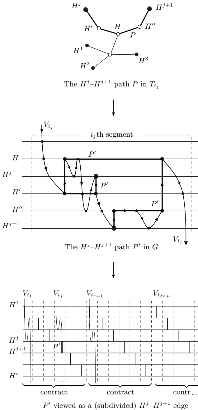
Fig. 12.4.4. An H^j-H^{j+1} path in T_{i_j} inducing segments of V_{i_j} for the j th edge of the grid's first vertical path
